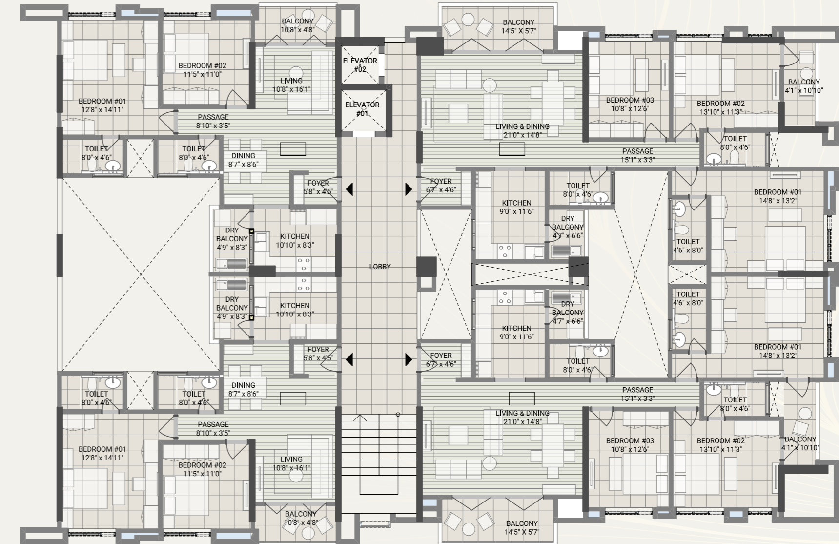
Typical floor plan phase 1
